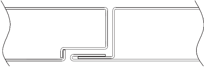
DOUBLE DOOR INTEGRAL ASTRAGAL
