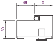
INTEGRAL FRAME SEAL
